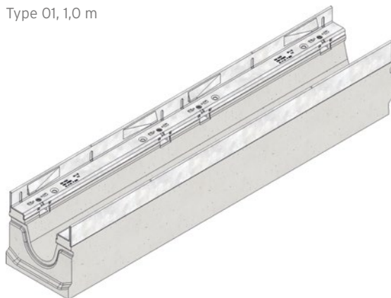
Type 01, 1,0 m
