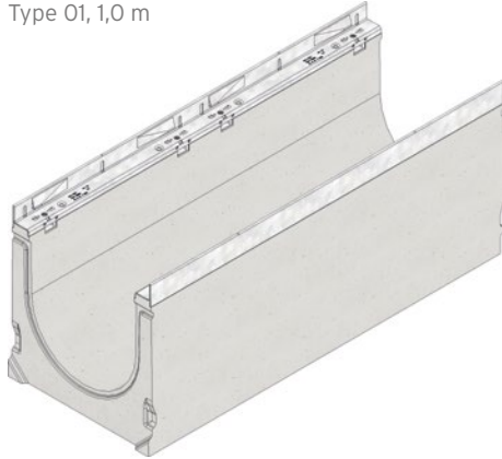
Type 01, 1,0 m
