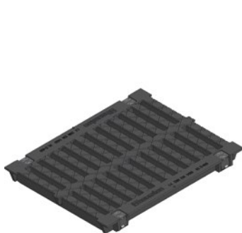
Ductile iron grating, SW 2 x 136/18 mm, black, with plastic caps, 0,5 m
