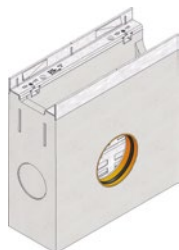
Trash box with galvanised mud bucket
