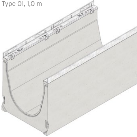
Type 01, 1,0 m
