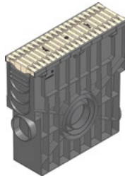
Trash box with PE mud bucket and FIBRETEC design slotted grating in the colour Sand SW 9 mm, class C 250, locked, 0,5 m
