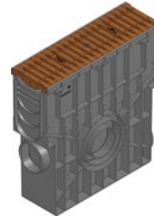
Trash box with PE mud bucket and FIBRETEC design slotted grating SW 9 mm, in the colour corten, class C 250, locked, 0,5 m
