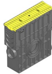
Trash box with PE mud bucket and FIBRETEC design slotted grating SW 9 mm, in the colour sun, class C 250, locked, 0,5 m
